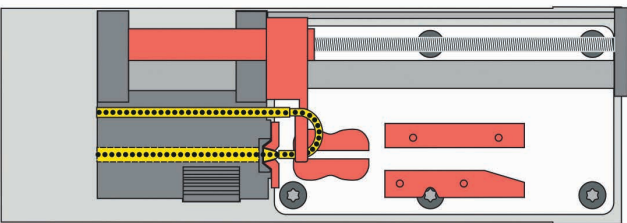
Switched-off LEIBINGER printer
